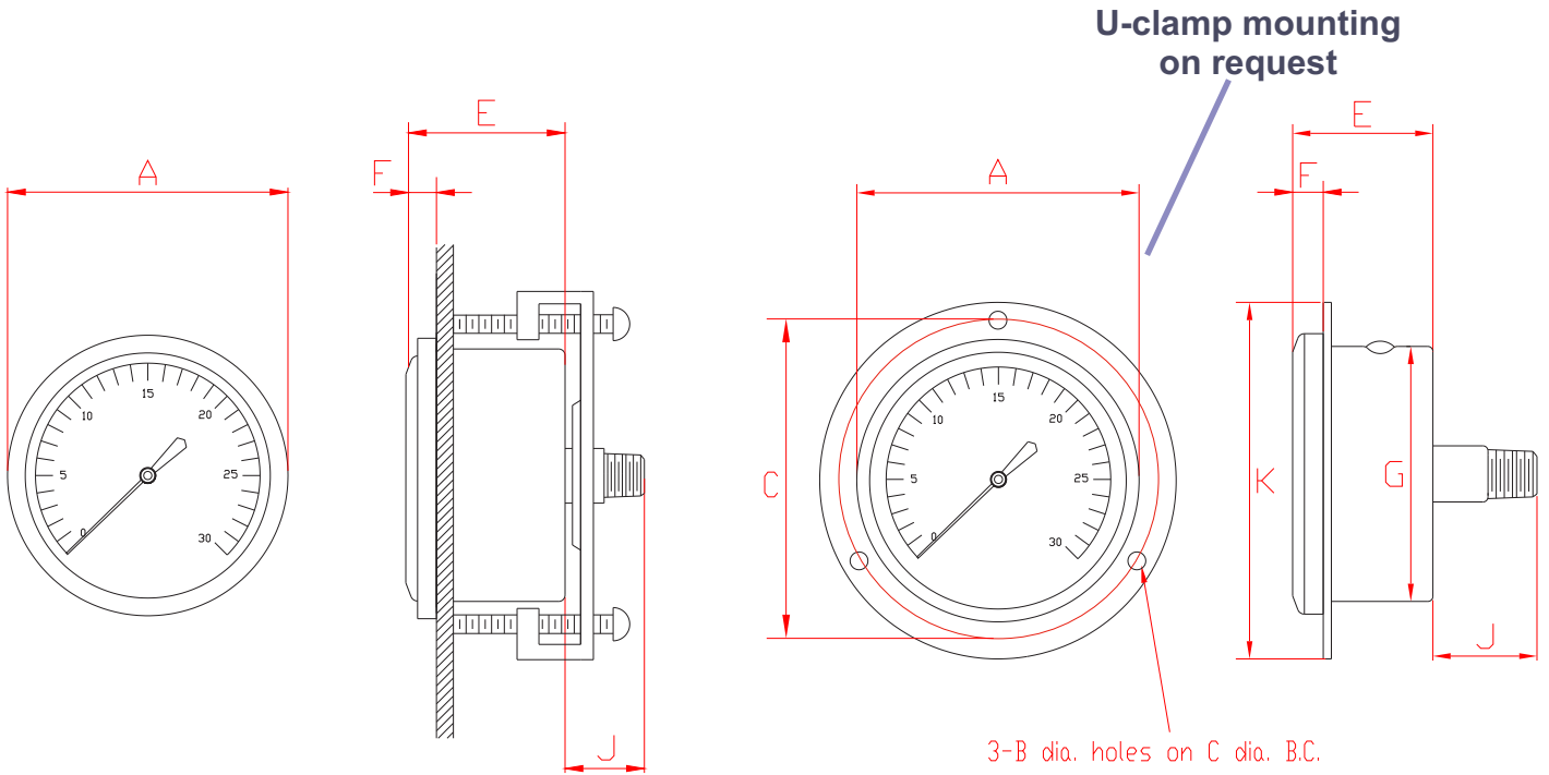
U-clamp
